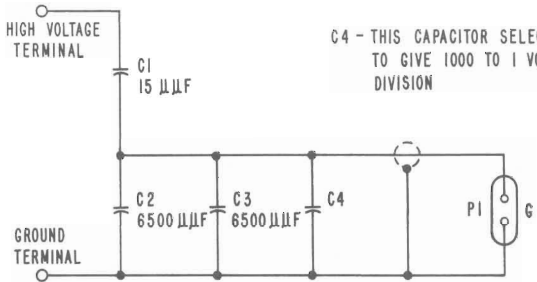
SCHEMATIC DIAGRAM OF MODEL 452 A
